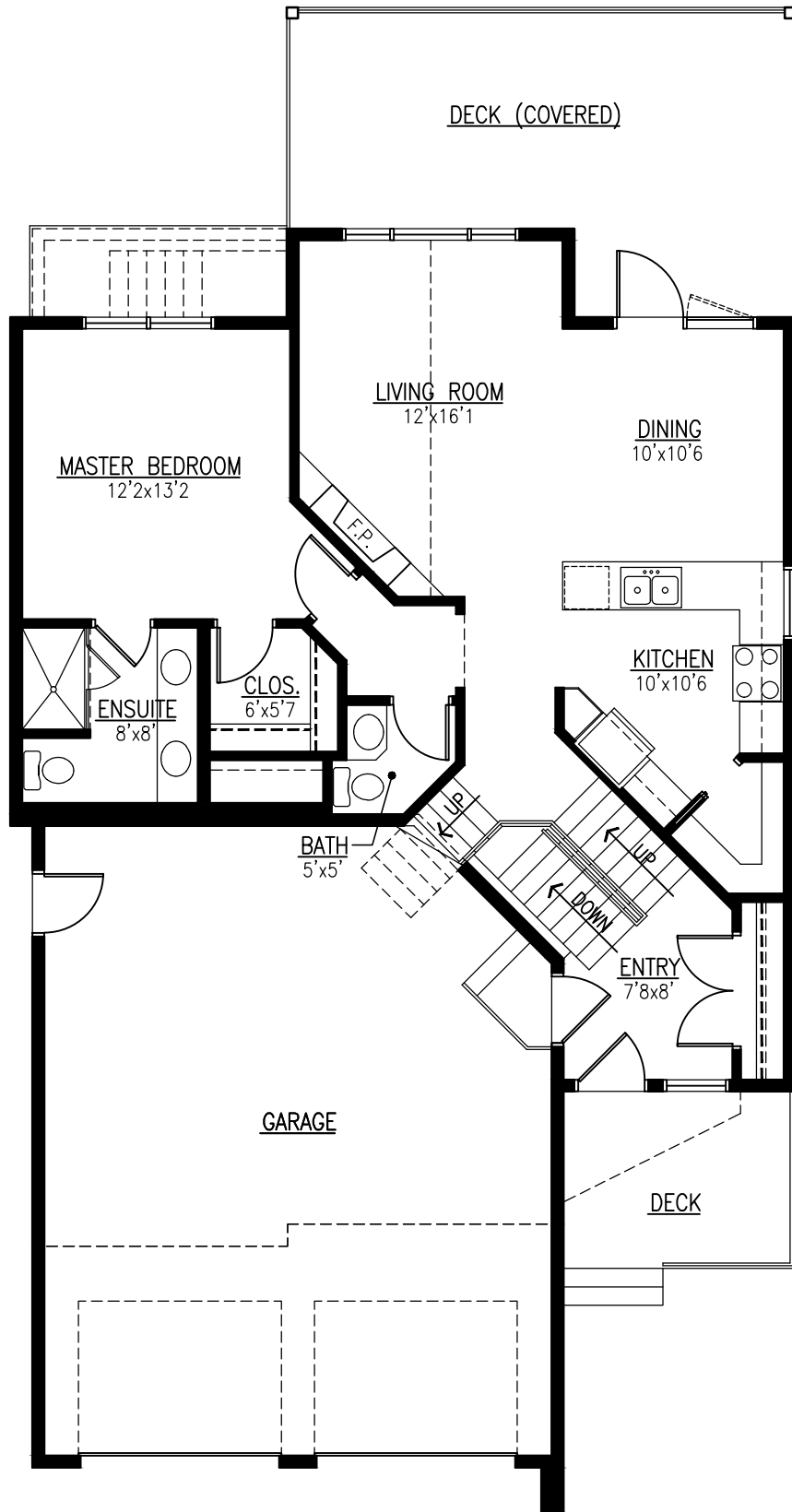
MAIN FLOOR PLAN 1008 SQ.FT.
